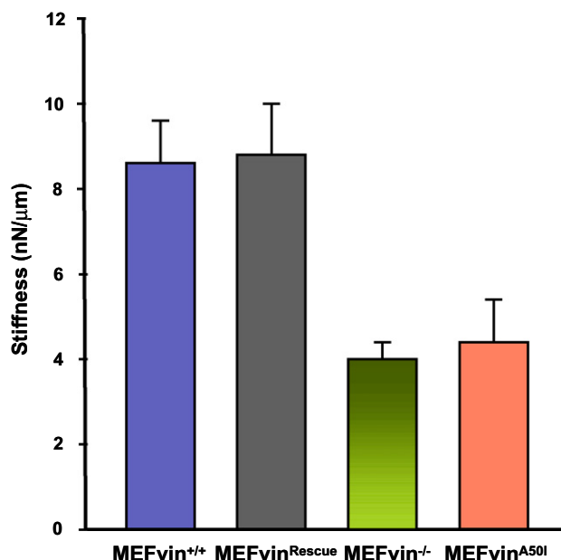
Fig. 1. Magnetic tweezer measurements of MEFvin +/+ (blue), MEFvin Rescue (black), MEFvin -/- (green), and MEFvin A50I (orange) cells. All cells were incubated with fibronectin-coated superparamagnetic beads (Ø 4.5 µm) for 30 min, after which the paramagnetic beads were displaced from their original position by 2 nN force of the magnetic tweezer. Displacement D(t) of the bead followed the relation, D(t) = 2 \text{ nN} \times a(t/t_0)^b , where the parameter 1/a (units of nN/µm) characterizes the cell stiffness. MEFvin +/+ and MEFvin Rescue cells were about twofold stiffer than MEFvin -/- and MEFvin A50I cells. The standard error of the mean (SEM) is indicated by the bars; the number of cells analyzed per cell line were between 65 and 85. (For interpretation of the references to color in this figure legend, the reader is referred to the web version of this article.)
