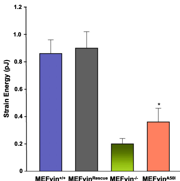
Fig. 2. 2D traction microscopy of MEFvin +/+ , MEFvin Rescue , MEFvin -/- , and MEFvin A50I cells. All cells were seeded on collagen-coated elastic substrates (~13 kPa) and tractions were determined. The strain energy of both MEFvin +/+ and MEFvin Rescue cells was about 4-fold higher than MEFvin -/- cells and approximately 3-fold higher than MEFvin A50I cells. The standard error of the mean (SEM) is indicated by the bars; the number of cells analyzed per cell line were between 30 and 80; * p < 0.05 .
